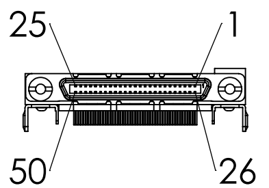
Connector Pinout (Female)
