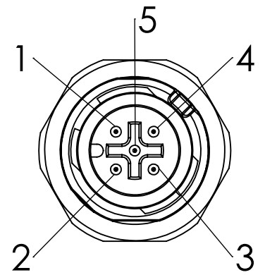
Connector Pinout (Male)
